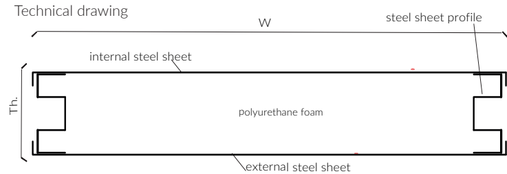
Technical drawing
