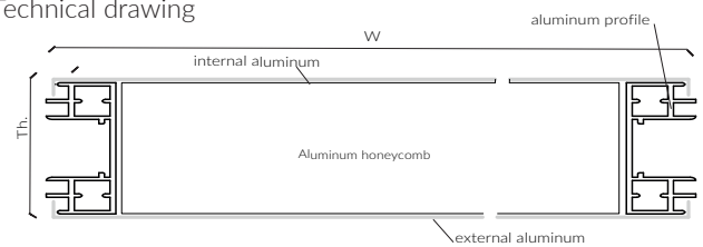
Technical drawing
