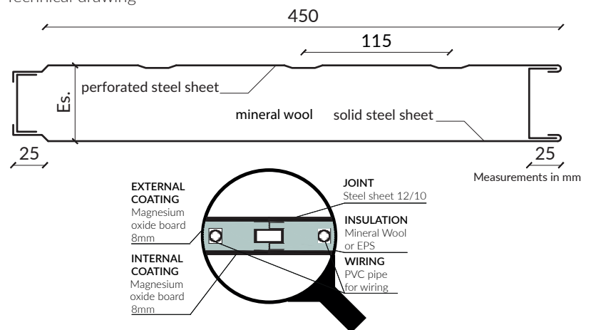
Technical drawing
